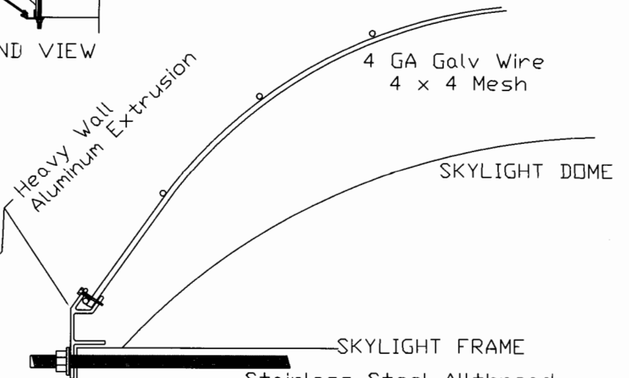
END SECTION 4X
