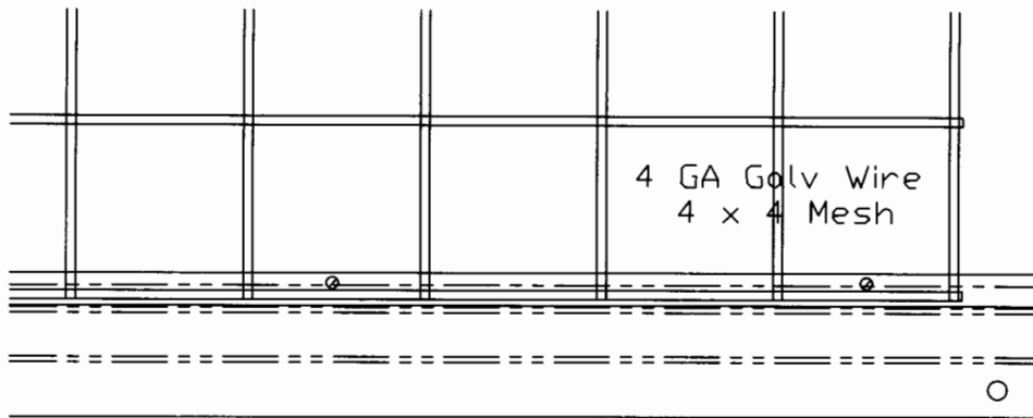
FRONT ELEVATION 4X
